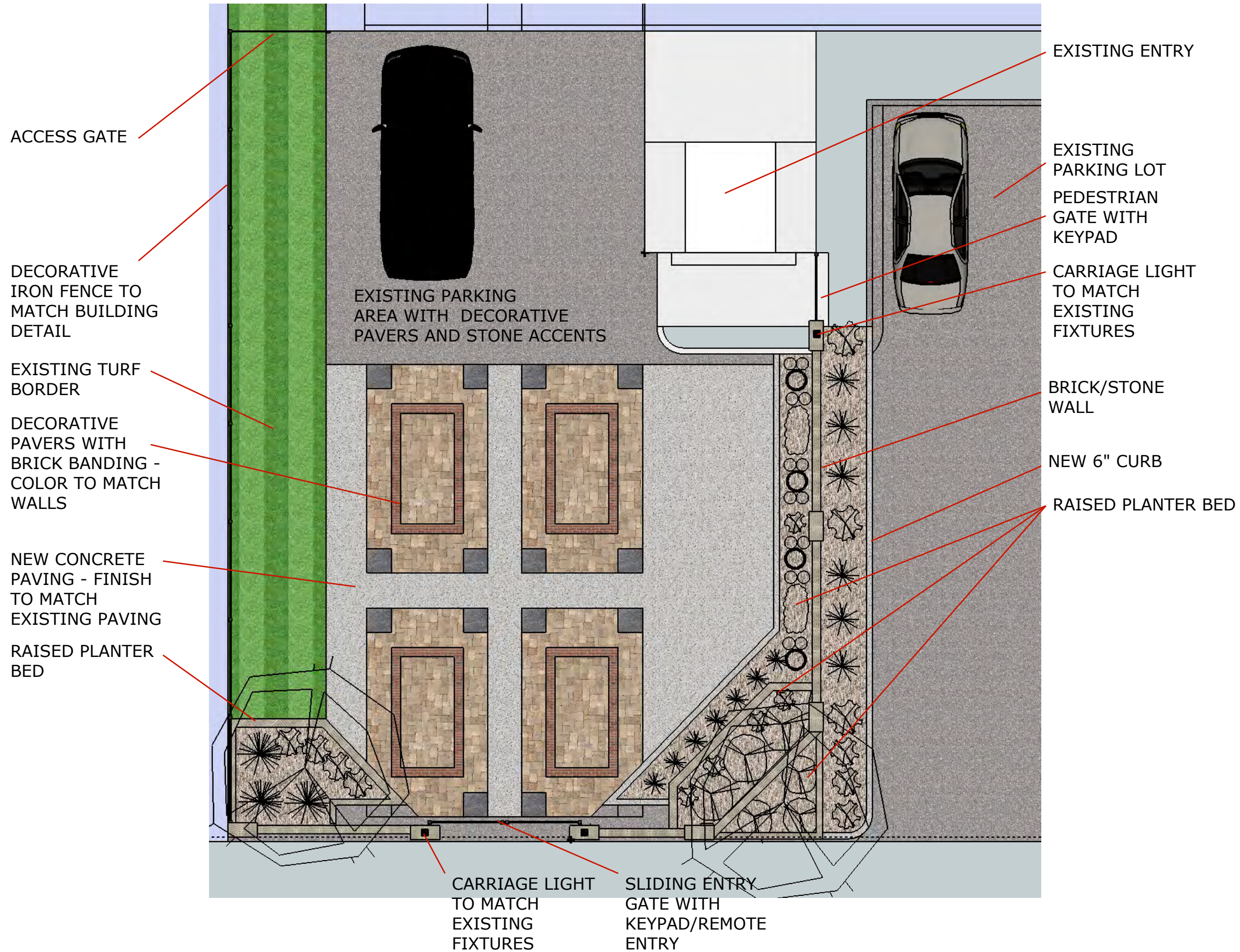
PLAN VIEW OF PROPOSED AUTO-COURT
